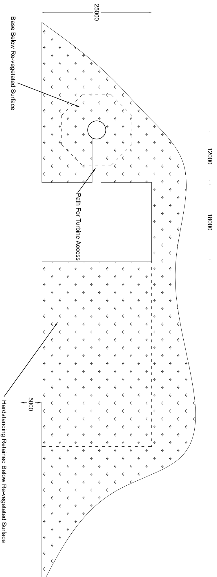
Re-vegetation to Hardstand Area Detail
